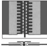
Alligator or Clipper Laced Seam
